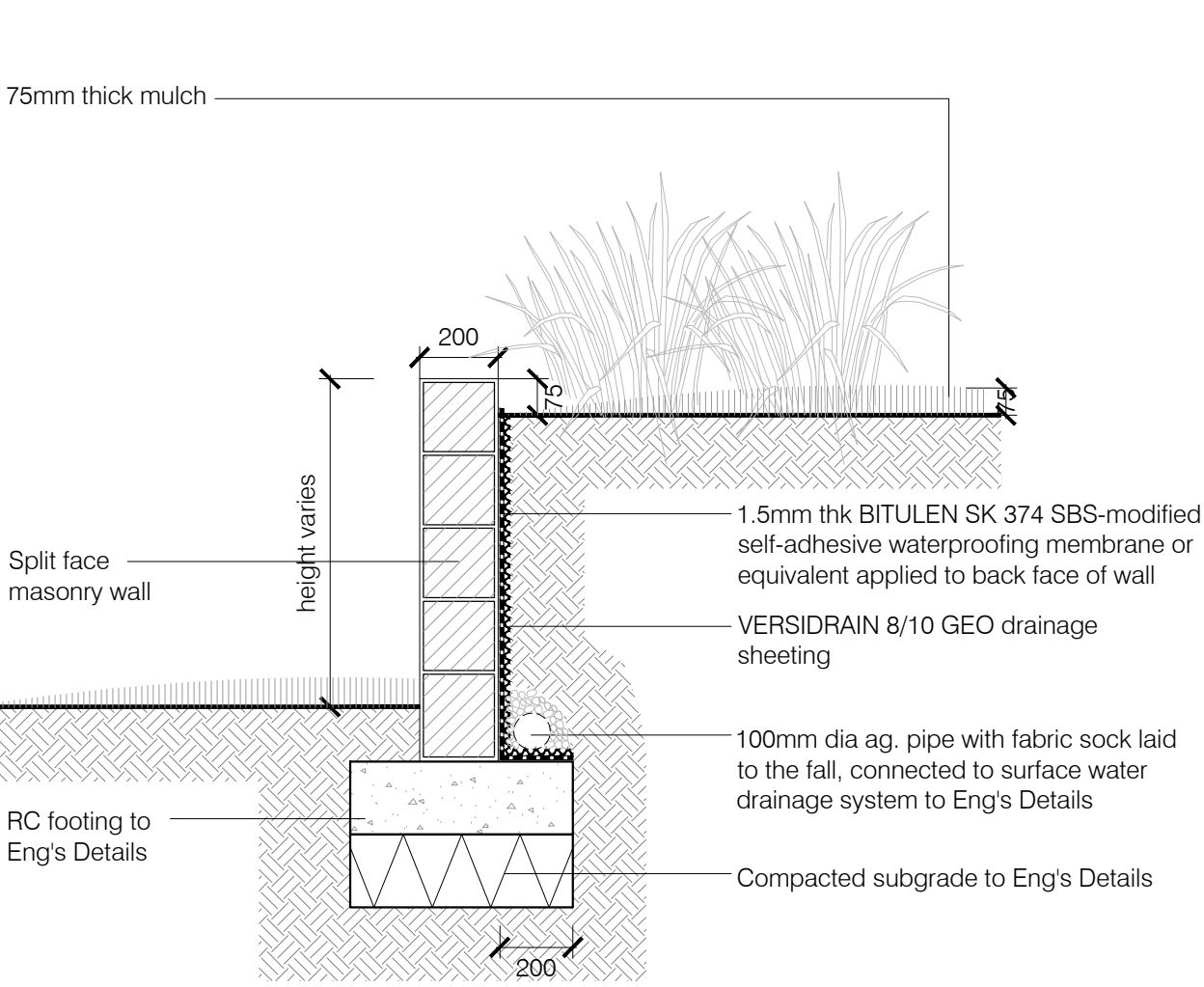
TYPICAL DETAIL 01: retaining wall scale: 1:20
