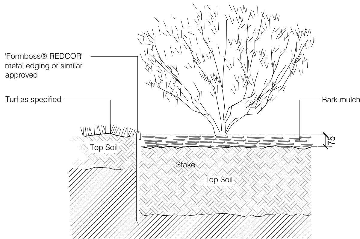
TYPICAL DETAIL 03: metal edging scale: 1:10
