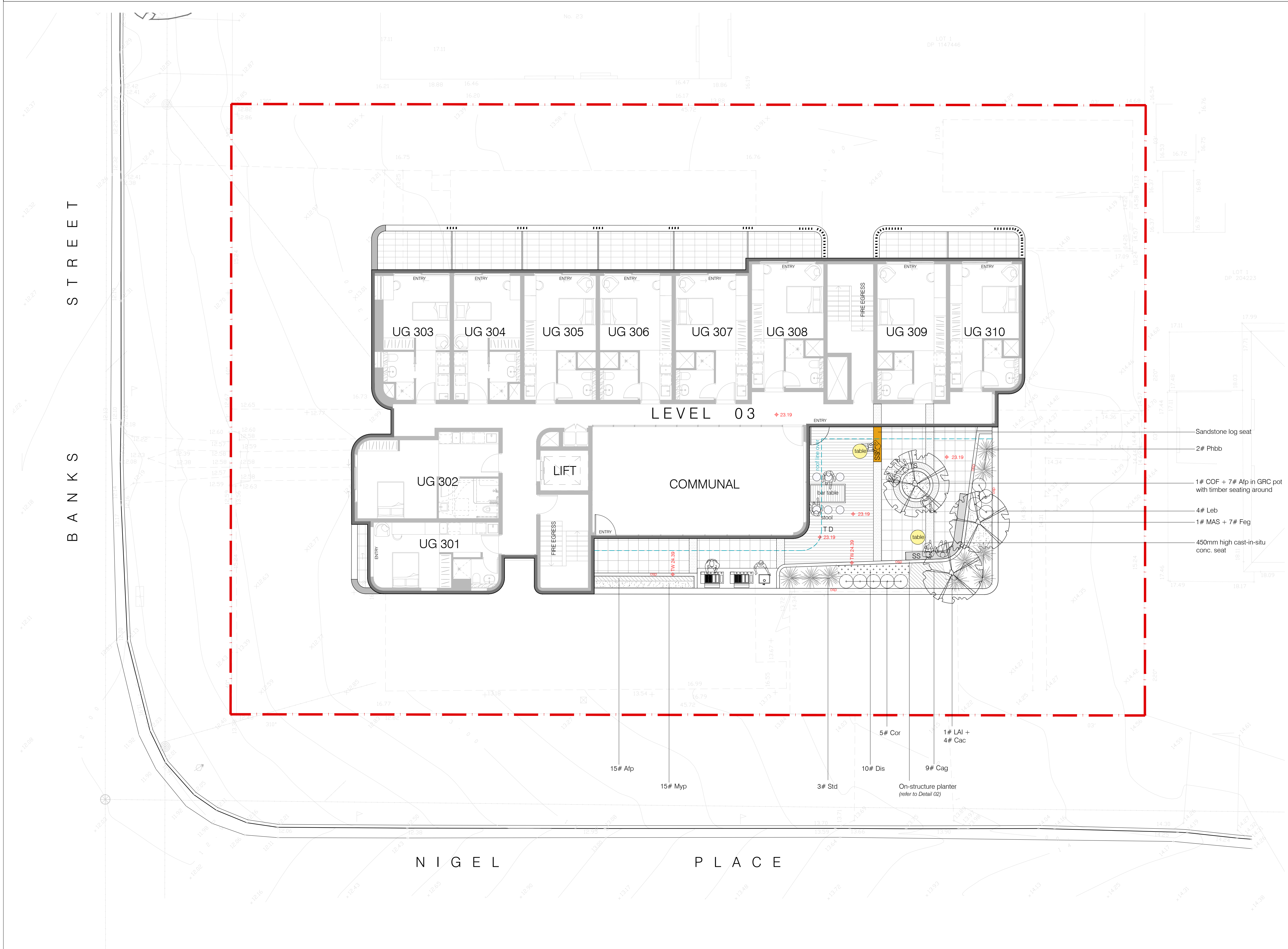
LANDSCAPE PLAN: level 03 scale: 1:100
