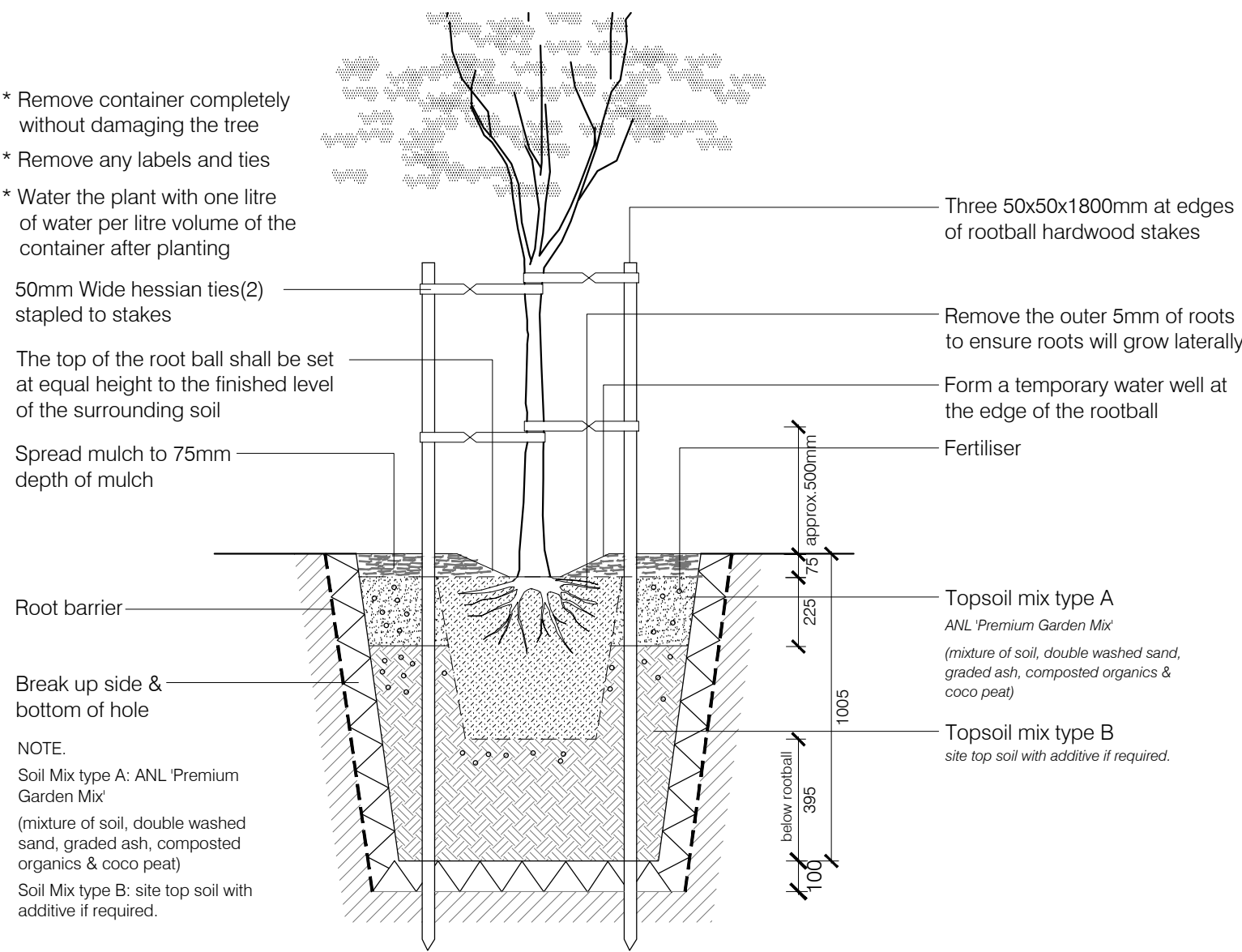
TYPICAL DETAIL 04: tree planting scale: 1:20
